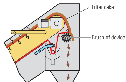
Endless belt with brush-of device
